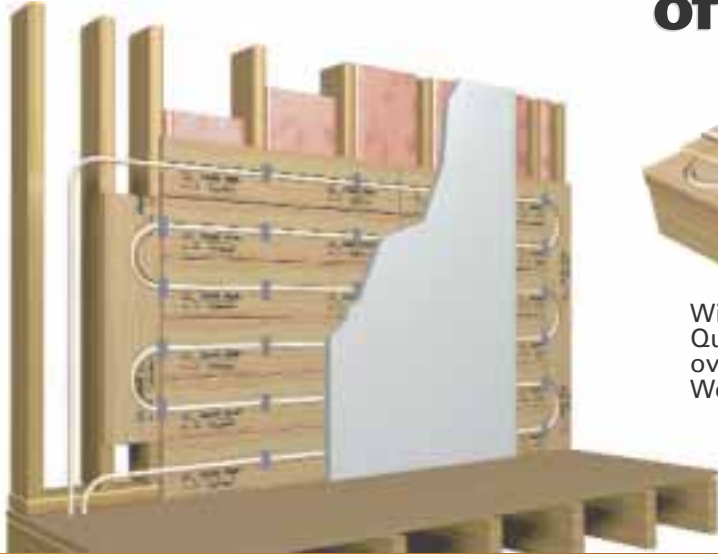
Wirsbo Quik Trak for Radiant Wall Heating
